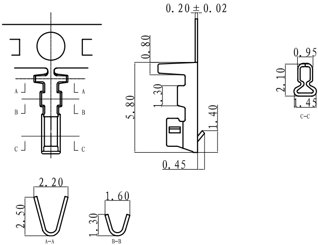
TERMINAL
