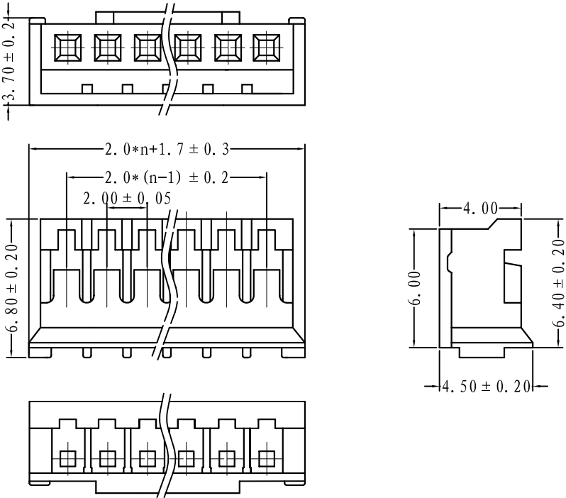
HOUSING
