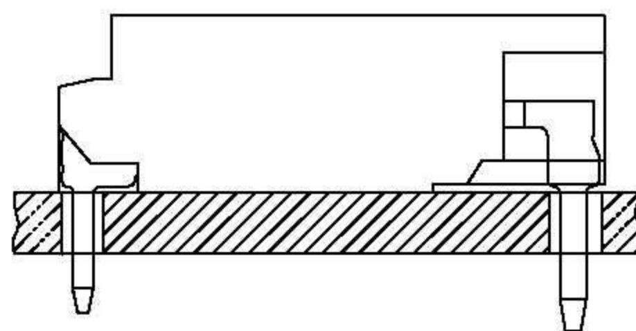
ASSEMBLY LAYOUT
