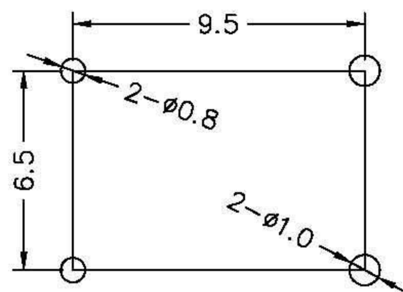
PCB LAYOUT
