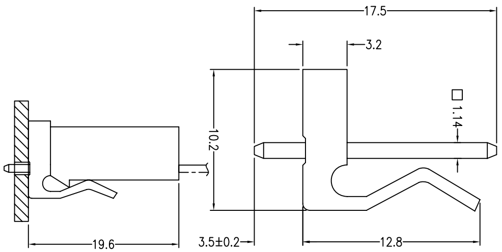
安装尺寸 MOUNTING MEASUREMENT
