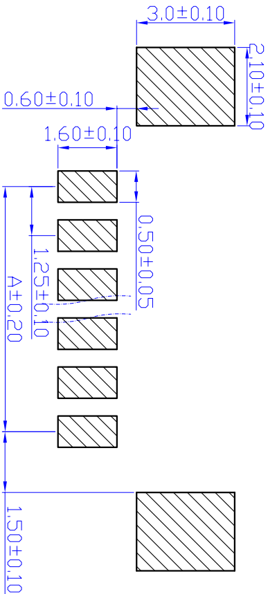
PCB Layout
